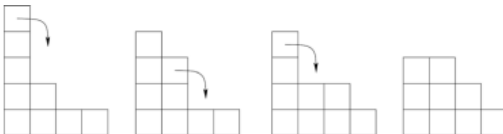
Figure 3 A discrete one-dimensional example of the evolution model. When the slope (difference in height in this case) is higher than a certain critical slope, some of the material moves to the shorter cell
